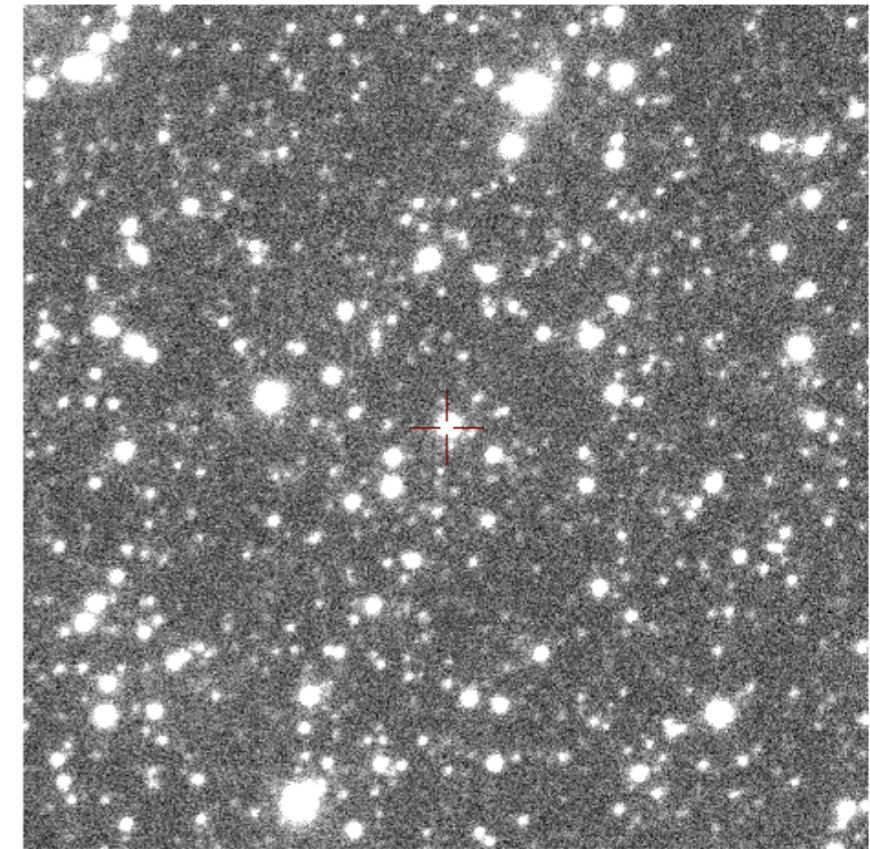
Image size 2' x 2'. North up, East left (OGLE-IV)
